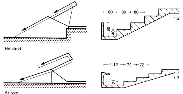
8 Stand profiles
